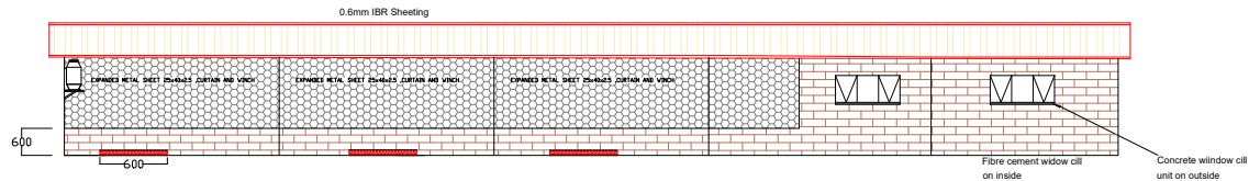
NORTH ELEVATION
