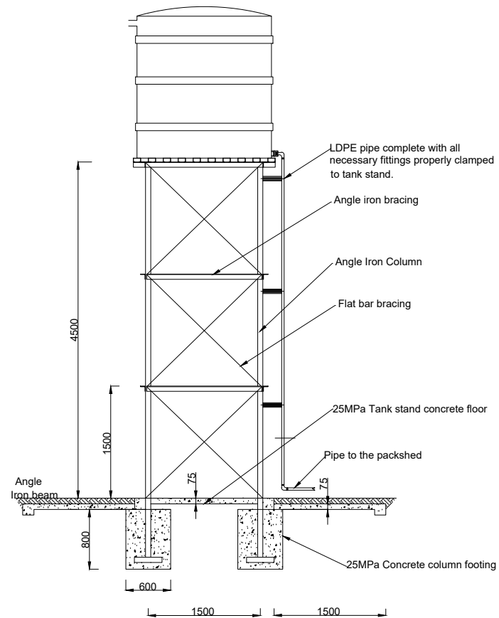
ELEVATION VIEW
