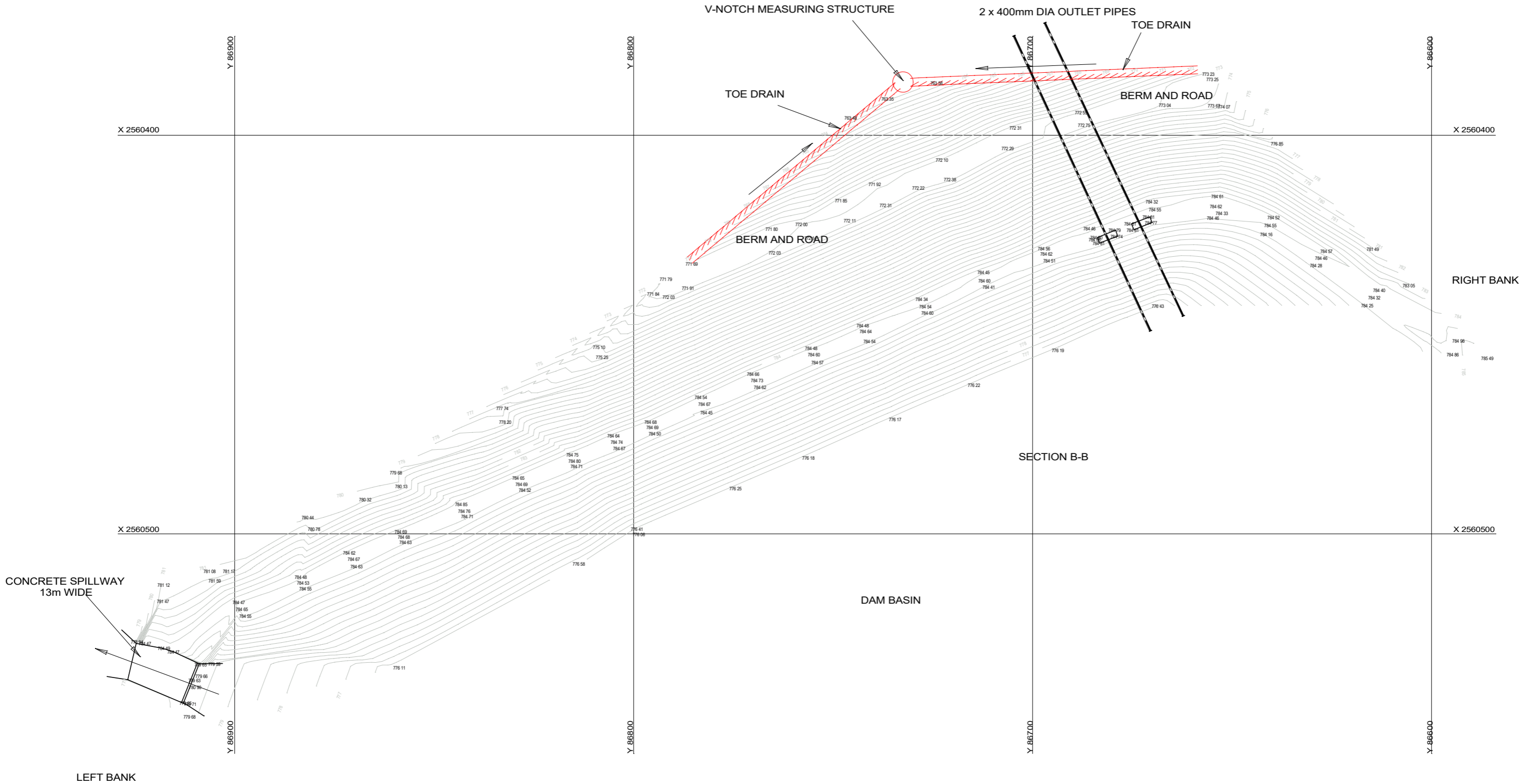
DAM WALL SURVEYED PLAN LAYOUT - SCALE 1:1000 (A3)
