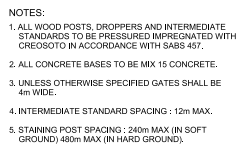
SPECIFICATION DRAWING 1.4m HIGH BARBED WIRE FENCE SCALE 1:100
