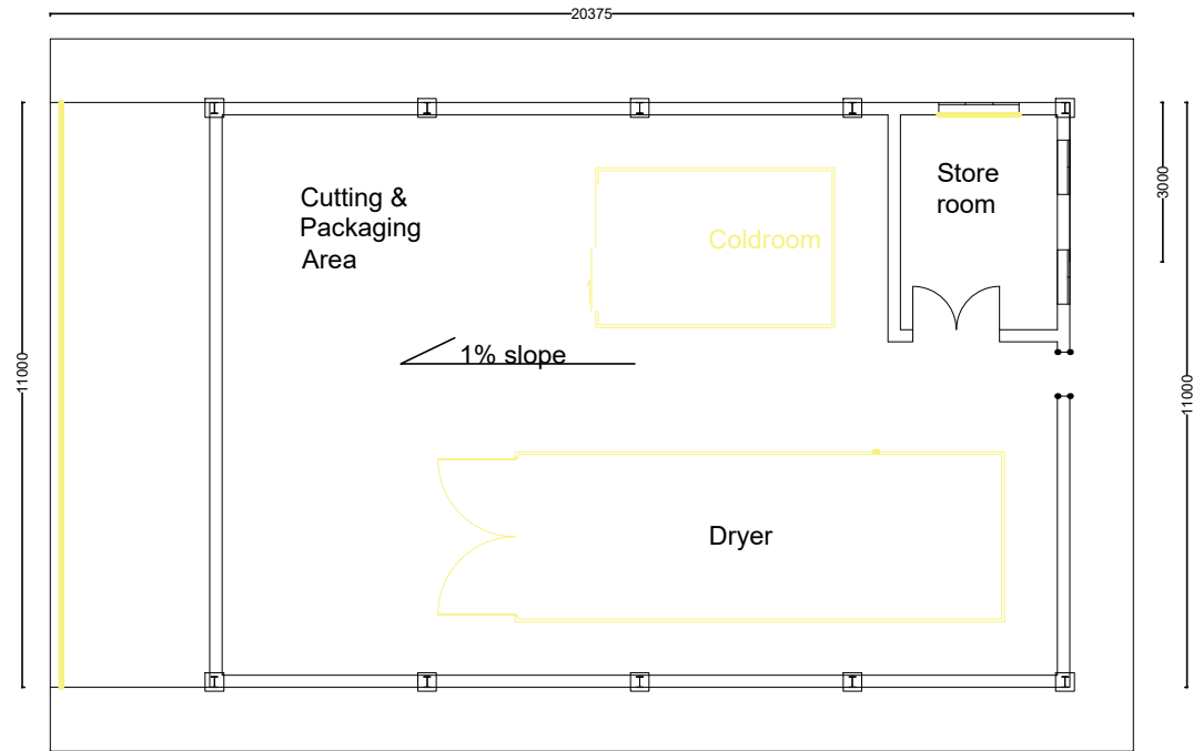
Foundation Layout
