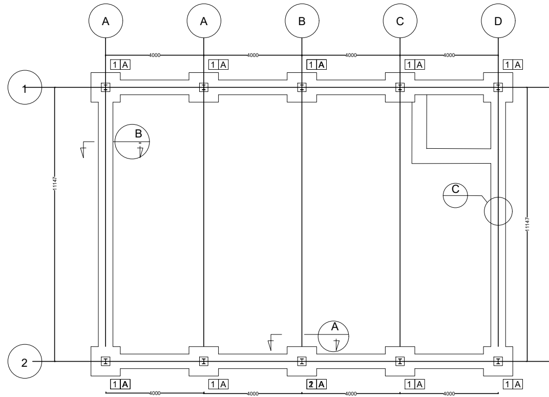
Plan Layout
