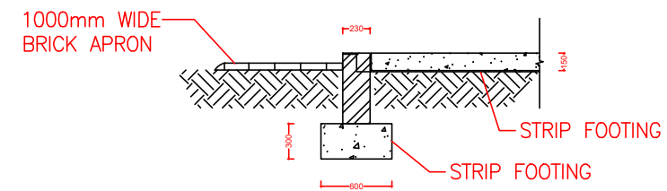
SECTION B
